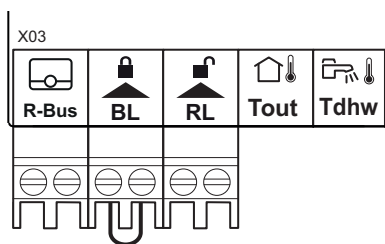
Afb.44 Connectors on the connection PCB
