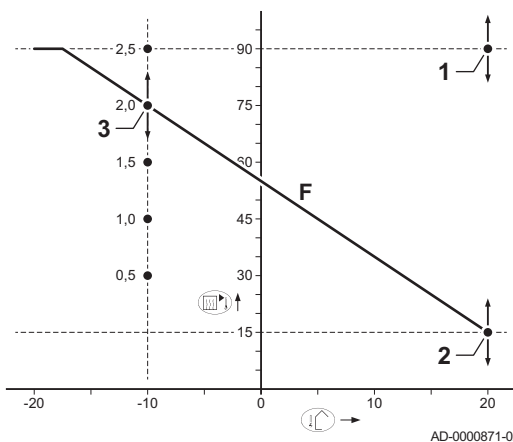
Afb.50 Interne stooklijn
