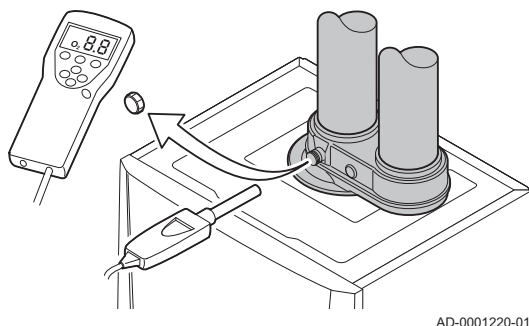
Afb.62 Rookgasmeetpunt
